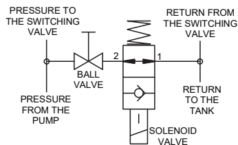
HYDRAULIC SCHEMATIC
