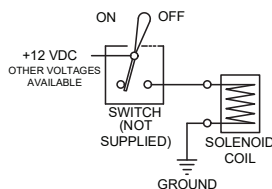
WIRING DIAGRAM
